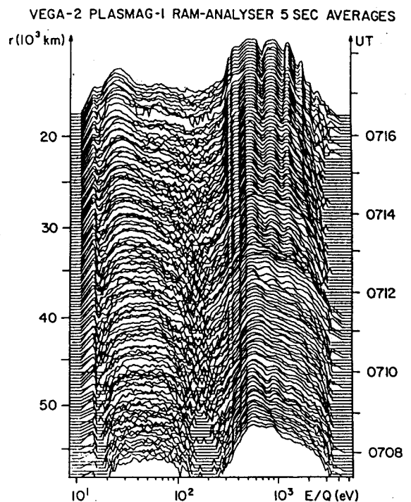
Fig. 3. Five second averages of the ram ion analyser spectra inside the cometary plasma region.
