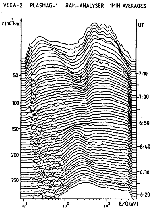
Fig. 2. One minute averages of the ram ion analyser spectra in the near cometary region.
