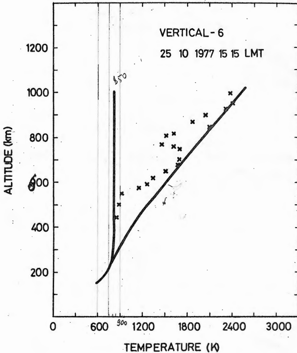
Fig.1 Variation of the neutral, ion and electron temperature with altitude at the time of apogee of the geophysical rocket "Vertical-6" computed on the basis of CIRA 1972, resp. the International Reference Ionosphere 1978. The measured ion temperature is denoted by crosses.
